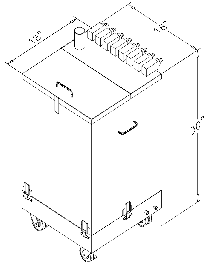
ISOMETRIC DETAIL OF HOPPER WITH TOP MOUNTED PUMPS AND 2" DIA. VENT SLEEVE
